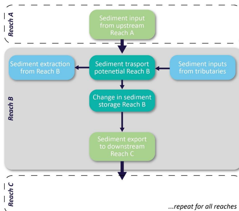
Figure 44. Diagram illustrating how the sediment inputs and sediment outputs are used to calculate change in sediment storage in each reach.
