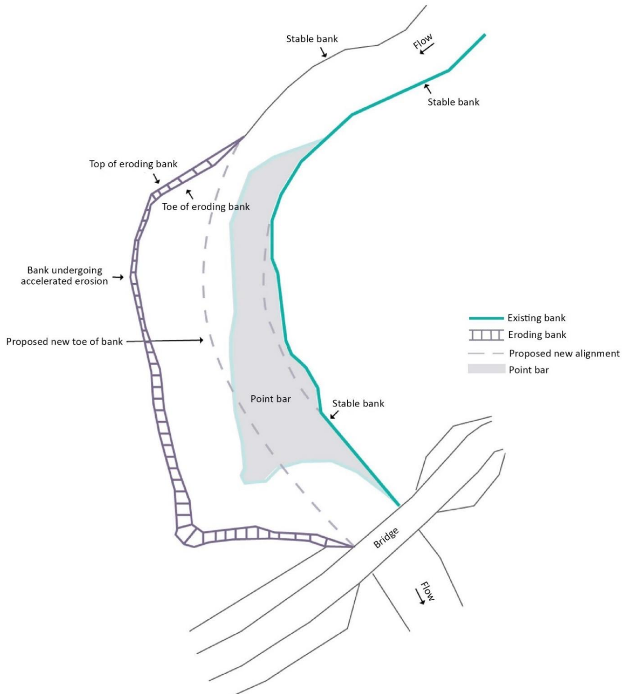
Figure 58. Pile field design – existing site layout.
