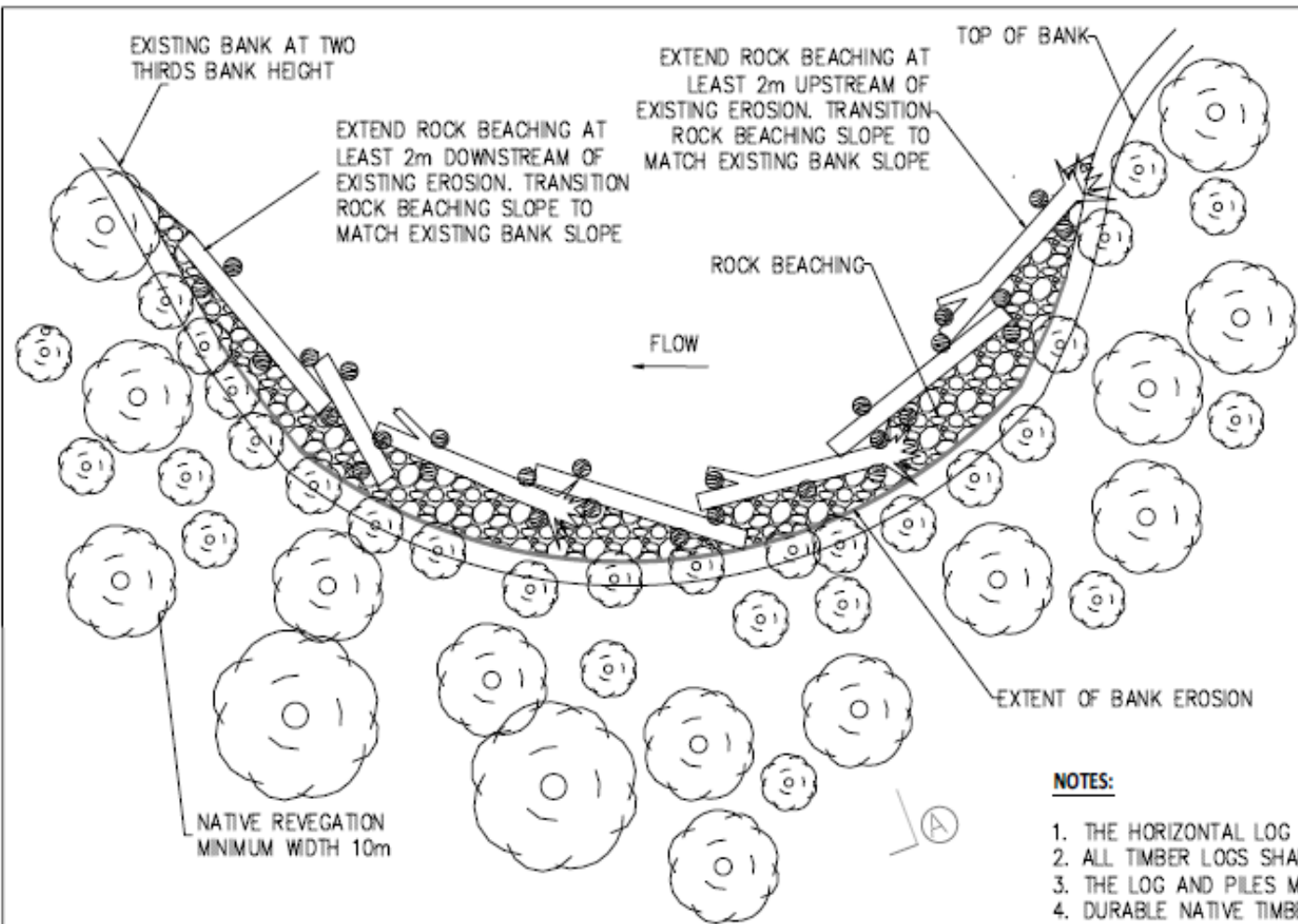
STANDARD PLAN VIEW
