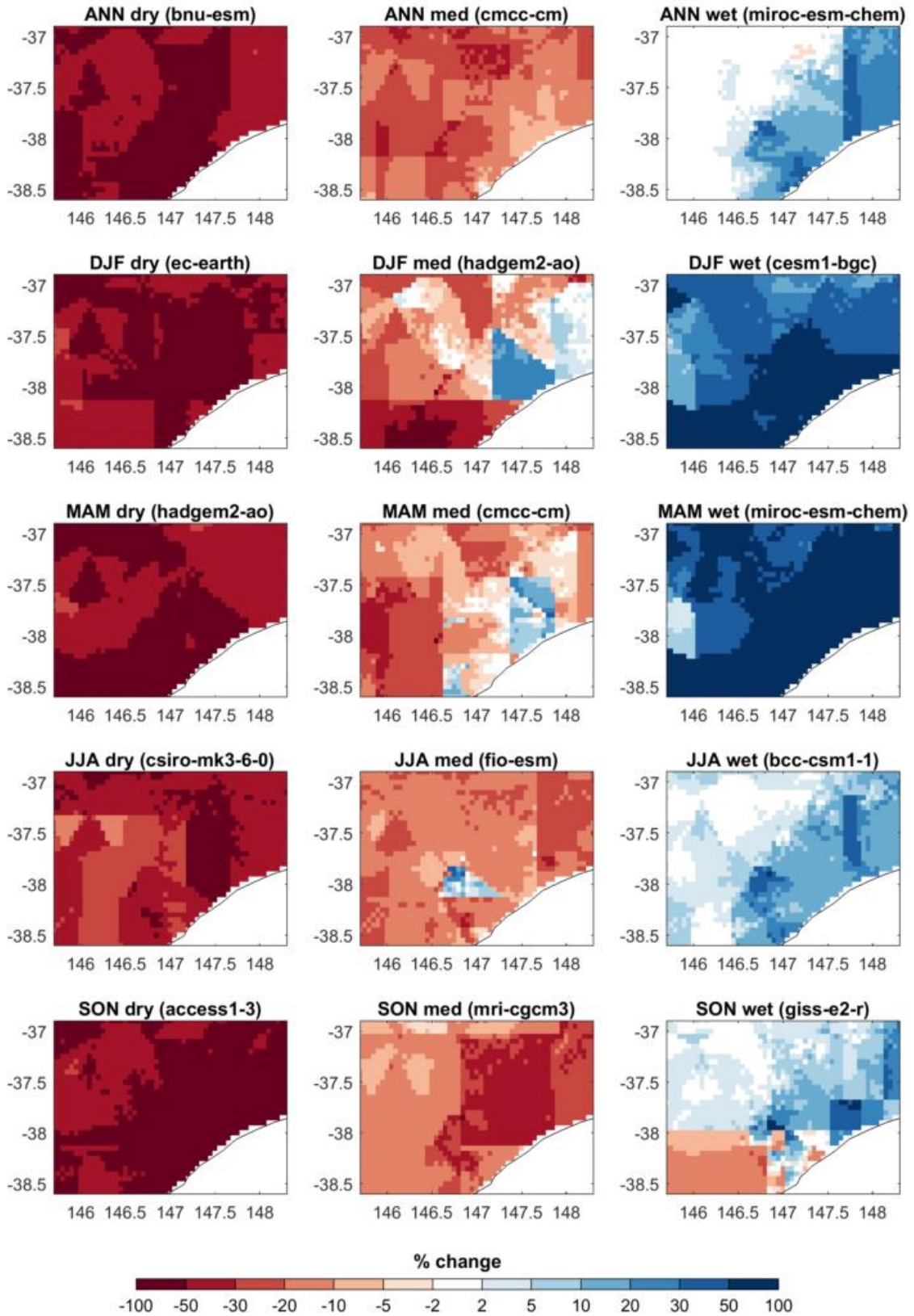
Figure 3.2 : Dry, median and wet change scenarios for runoff under RCP8.5 for the future period centred on 2065 over the LVRSS region. ANN: annual change; DJF: December-January-February; MAM: March-April-May; JJA: June-July-August; SON: September-October-November. The GCM that represents each scenario is given in brackets.
