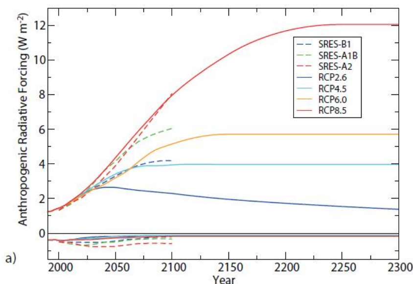
Figure 4.1 : The radiative forcing (enhanced greenhouse effect) under the Representative Concentration Pathways, showing greenhouse gas (positive) and aerosol (negative) forcing. The previous generation SRES scenarios are also shown for reference. Source: IPCC AR5 Chapter 12 (Collins et al., 2013)
