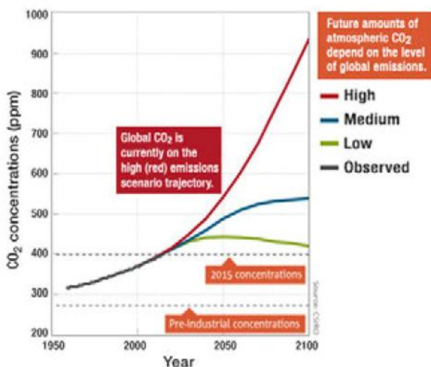
Figure B.1 : Future greenhouse gas emissions scenarios
