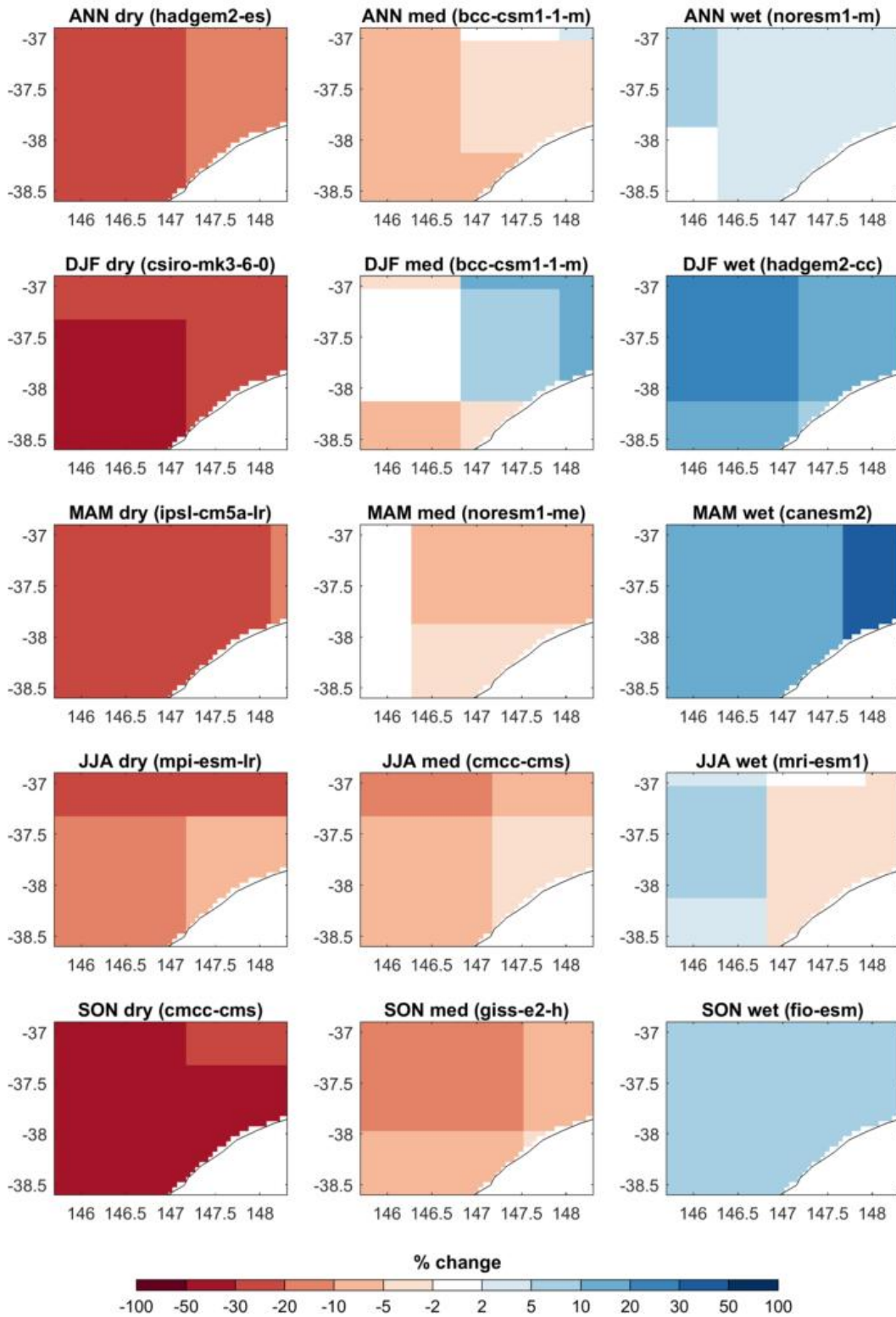
Figure 3.1 : Dry, median (med) and wet change scenarios for rainfall under RCP8.5 for the future period centred on 2065 over the LVRSS region. ANN: annual change; DJF: December-January-February; MAM: March-April-May; JJA: June-July-August; SON: September-October-November. The GCM that represents each scenario is given in brackets.
