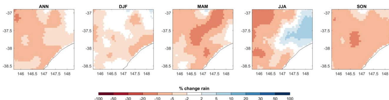
Figure 3.3 : Change in mean rainfall from 1975-2014 to 1997-2014. ANN: annual change; DJF: December-January-February; MAM: March-April-May; JJA: June-July-August; SON: September-October-November.
