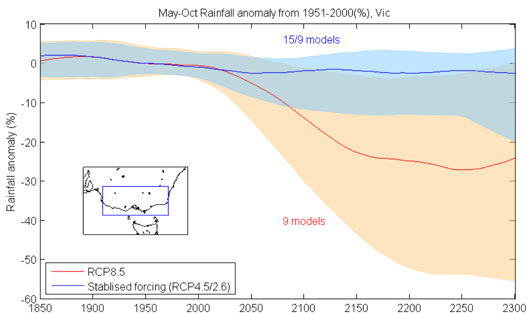
Figure 4.4 : Rainfall projections from CMIP5 GCMs for May-October within the box as marked, for RCP8.5 and RCP4.5/2.6 combined. The line shows the median of models, shading shows the 10-90% range of models using the number of models for each ensemble as marked.
