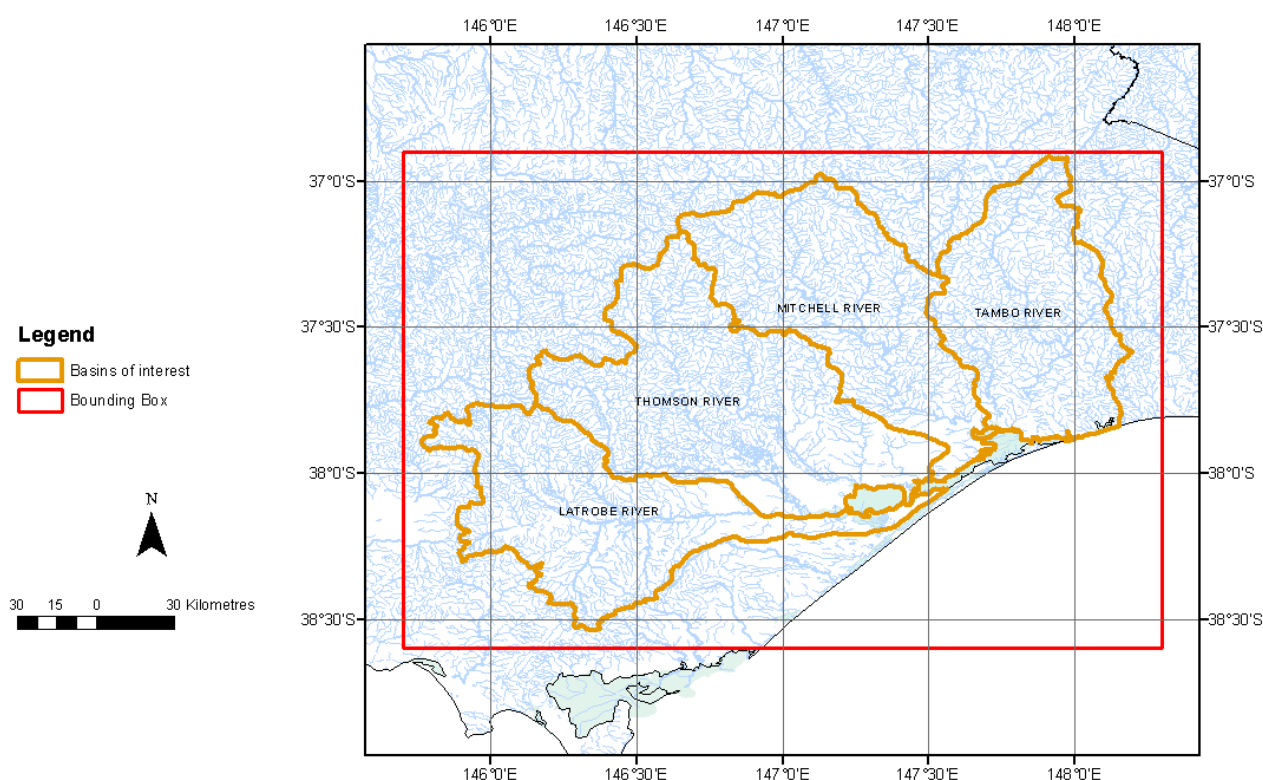
Figure 2.1 : Gippsland domain (red square) and basins (orange boundaries) for which GCM outputs are ranked to identify dry, median and wet scenarios.
