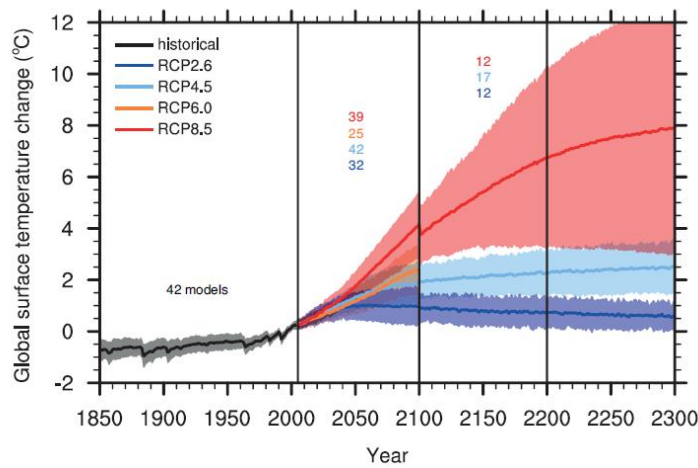
Figure 4.2 : Global temperature change relative to 1986-2005 from CMIP5 global climate models under historical and RCP simulations. Lines show the median of model simulations, shading shows 5-95% of the model range. The number of models in each simulation is indicated by the coloured numbers.
