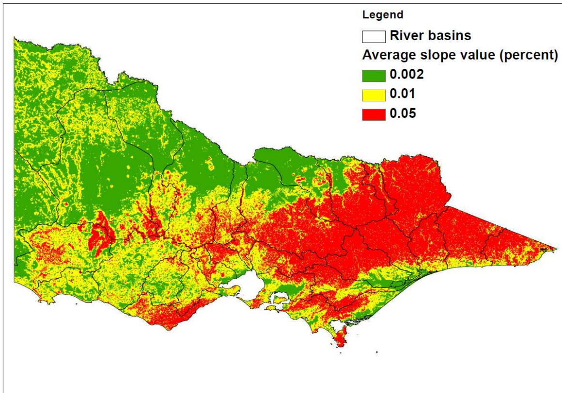
Figure 2-3 Victoria statewide slope map
