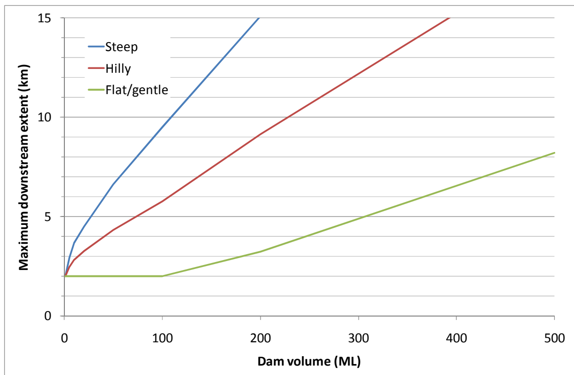
Figure 2-2 Indicative maximum downstream extent of dambreak impact
