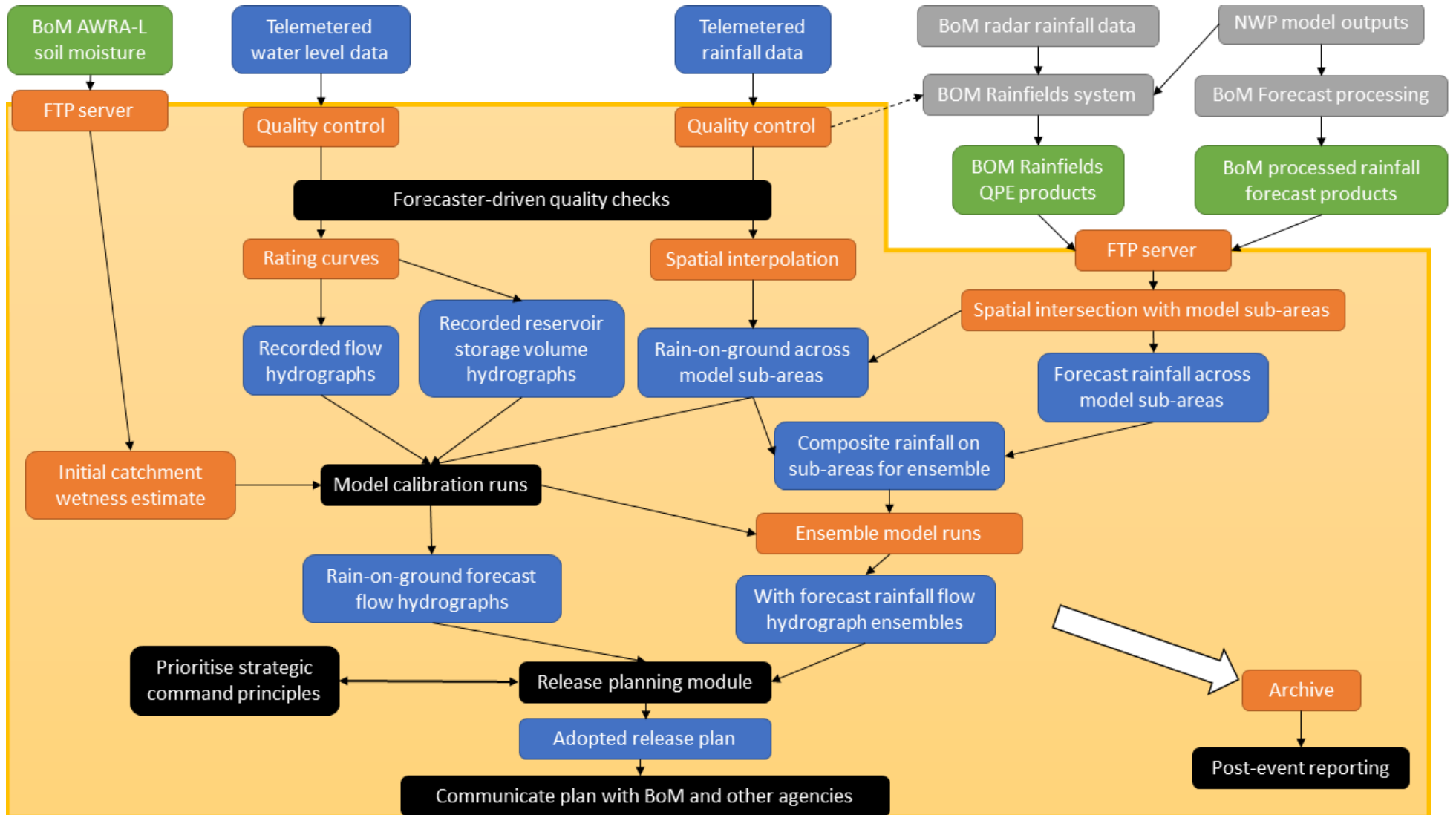
Figure 5-5 Integrated flood forecasting system for dam operations, for a system implementing rain-on-ground and rainfall forecast generated flows
