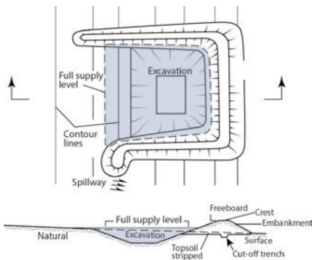
Figure 4.3 – Off-stream storage (hillside dam).
