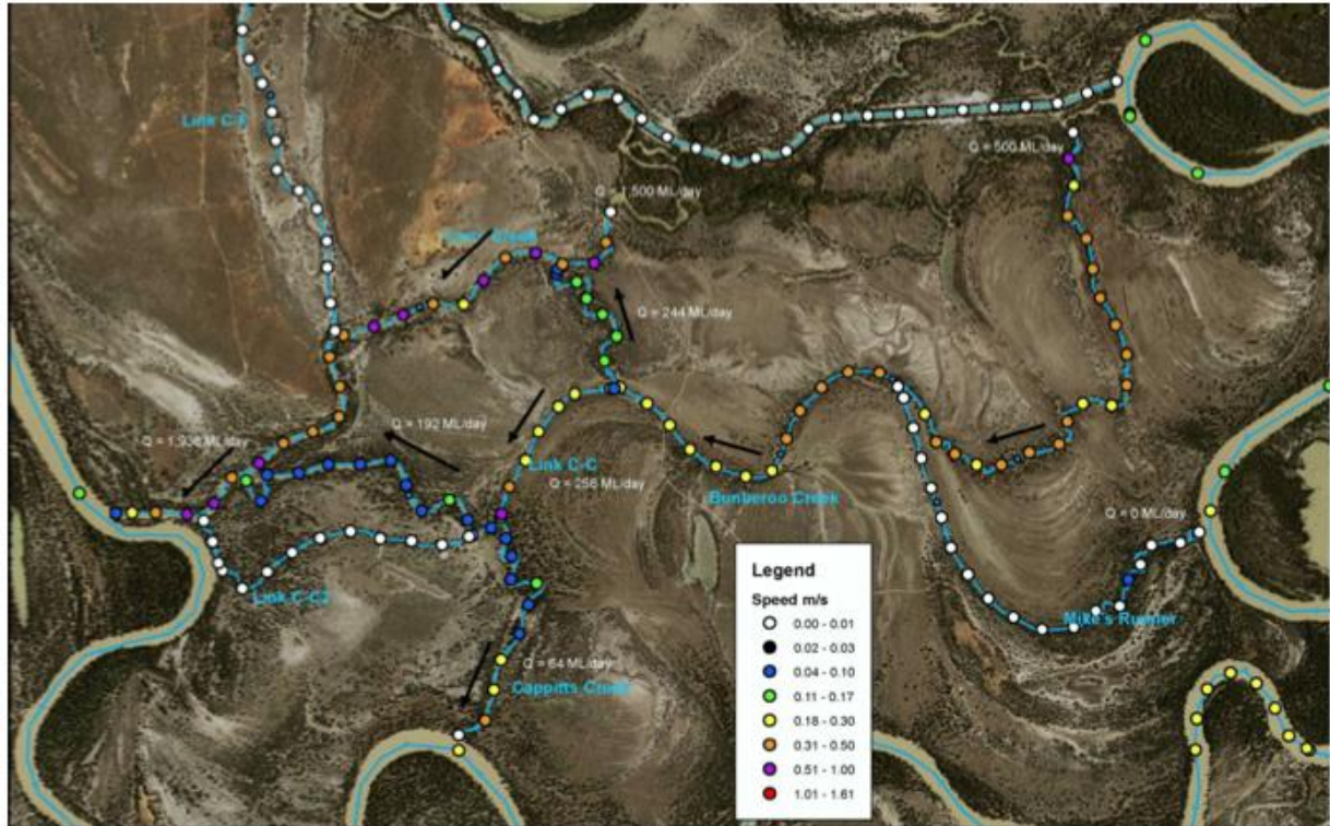
Figure 25. Hydrodynamic modelling of CCB system showing mean velocity within the channel with inflows of 1,500 ML/d at Carrs No. 1 and 500 ML/d at Carrs 2 (Robinson and Mallen-Cooper 2013).
