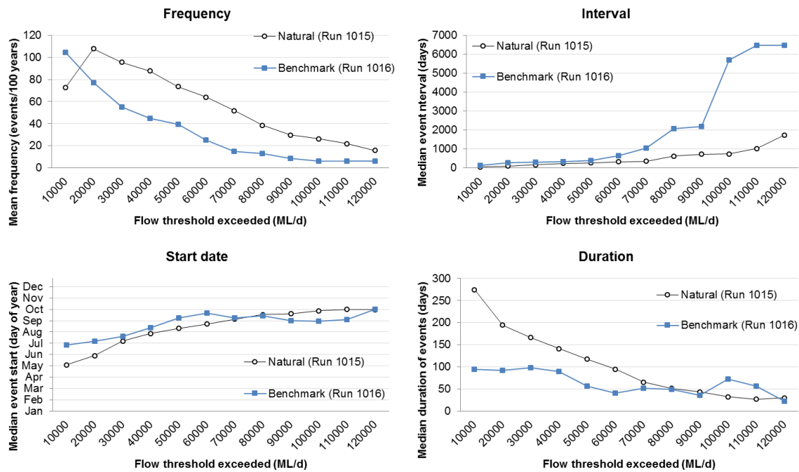
Figure 11. Spells analysis for Murray River flows upstream of Lock 9 for natural and Benchmark scenarios over a 114 year modelled period (Fluvial Systems 2014)
